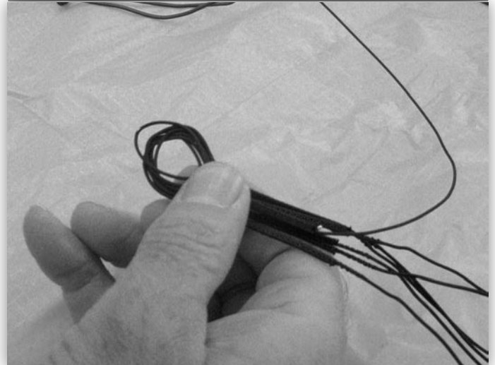
fig. 4 - Add the limiter line loop next to the bridle line loops. The limiter line should run in the same direction as the other bridle lines.
