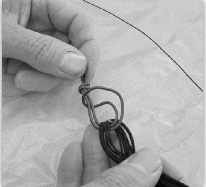
fig. 6 - Larkshead knot the bridle toggle onto the bridle loops.
