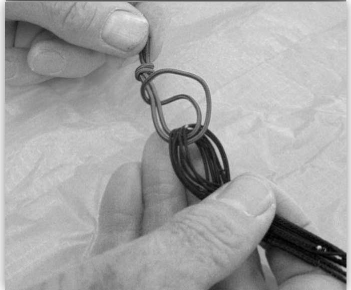
fig. 2 - Detach the bridle toggle from the bridles. Simply loosen the larkhead knot and remove.
